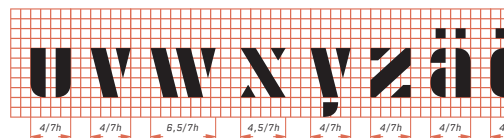
Schablenschrift A (Stecil Type A) constuction template, blueprint
